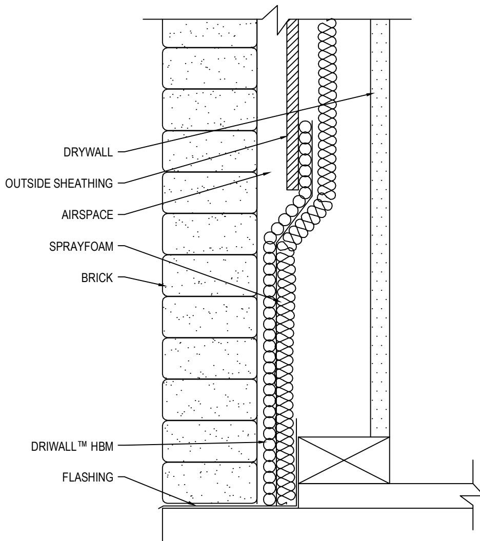
SECTION VIEW
